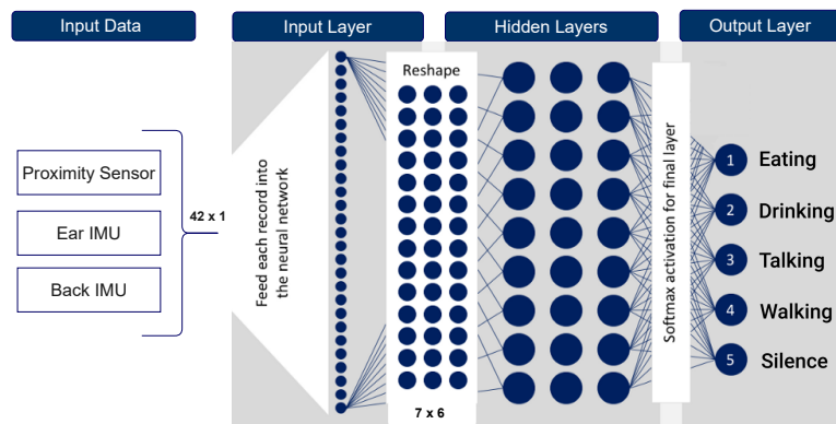
Fig. 6. FitNibble's DNN model topology.
