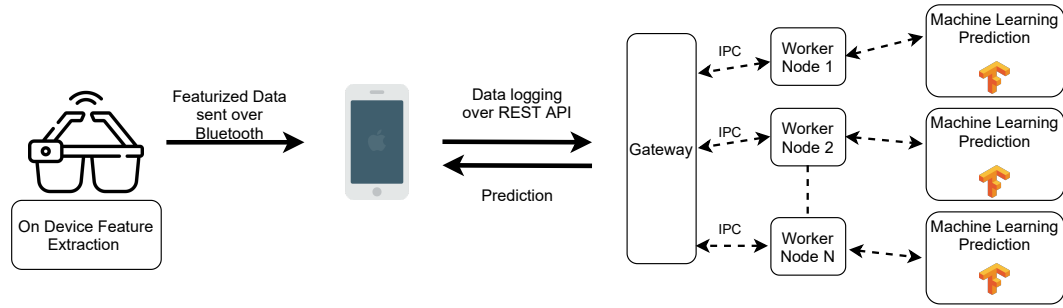
Fig. 2. System architecture: FitNibble wearable sends the extracted features over Bluetooth to our iOS mobile App. The backend obtains this data over REST API and then forwards it for data logging and model prediction of eating.
