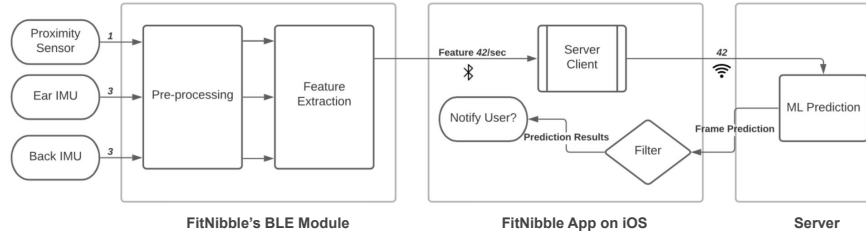
Fig. 4. The flow of data and information across the the three main components of the end-to-end system.
