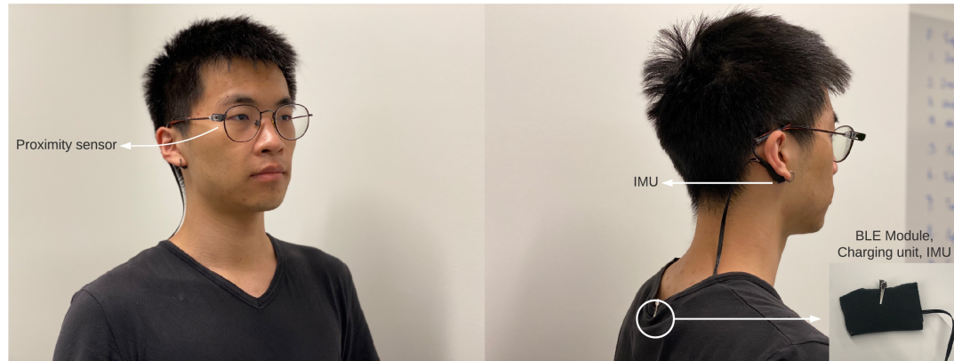
Fig. 3. The wearable has a proximity sensor to detect hand-to-mouth gestures (left), an IMU in contact with the lower jaw bone to detect chewing (right), and small cloth pocket clipped to the back of the user's shirt containing the BLE module, battery, and the reference IMU (bottom right).
